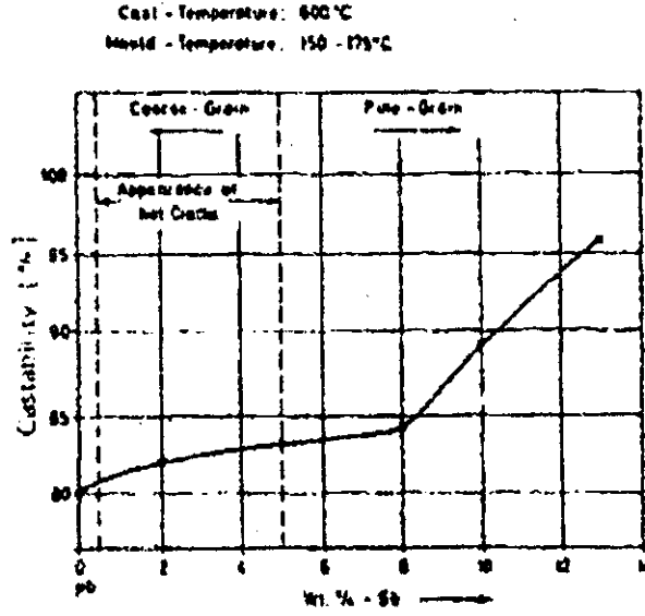
Castability of lead- antimony alloys.
