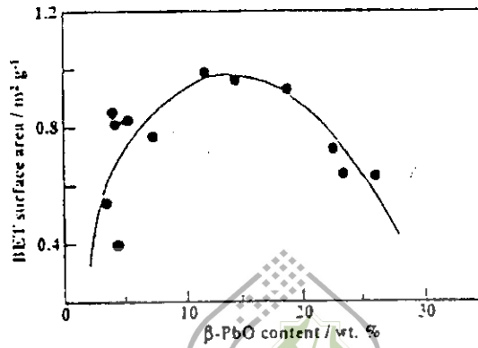
. Influence of β-PbO content on surface area of leady oxide.
