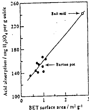
1. Reactivity of bail-mill and Barton-pot lead oxides [16].
